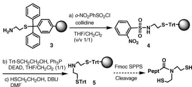
Scheme 3. Synthesis of C-Terminal BMEA Peptides
