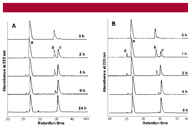
Figure 2. Ligation between H-LKSFG-BMEA and H-CLKFA-NH 2 in the presence of MESNa (2% w/v) and 50 mM TCEP and at pH 5. HPLC gradient: 0–50% buffer B in 50 min. (A) Reaction at 37 °C. (B) Reaction under microwave irradiation. Peak a, H-CLKFA-NH 2 ; peak b, H-LKSFG-BMEA; peak c, ligation product; peak d, H-LKSFG-MES thioester.
