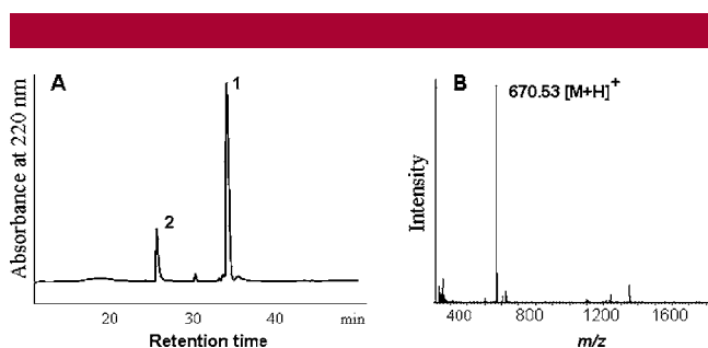
Figure 1. HPLC (A) and MS (B) analyses of LKSFG-BMEA. Peak 1, amide form; peak 2, thioester form. HPLC gradient: 0 – 45% buffer B in 45 min.
