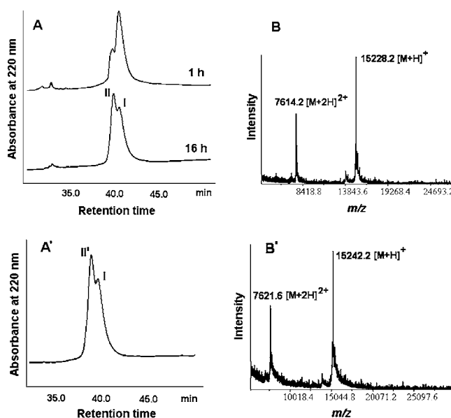
Figure 3. (Top half) Synthesis of histone H3/K14C through ligation between H3(1–13)-BMEA and H3(14–135)/K14C under microwave irradiation. (A) HPLC monitoring of the ligation reaction; (B) MALDI MS of the isolated ligation product H3/K14C (MW calcd 15227.7). (Bottom half) Synthesis of a histone H3 analog H3/K4me-K14C through ligation between H3(1–13)/K4me-BMEA and H3(14–135)/K14C at 37 °C. (A') HPLC monitoring of the ligation reaction at 2 days; (B') MALDI MS of the isolated ligation product (MW calcd 15241.7). Peak I, unreacted H3(14–135)/K14C ; peak II or II', ligation product. The BMEA peptide eluted out much earlier before the HPLC range shown here.
